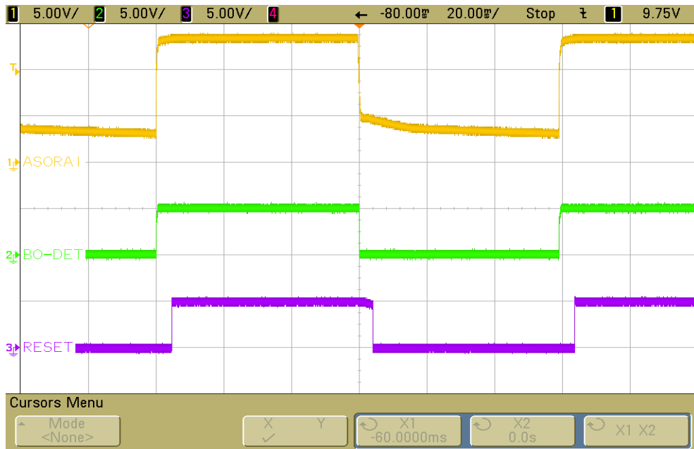
Figure 33. BO-DET Response to LOW Voltage – VBAT-MON tied to ASO-RAIL
